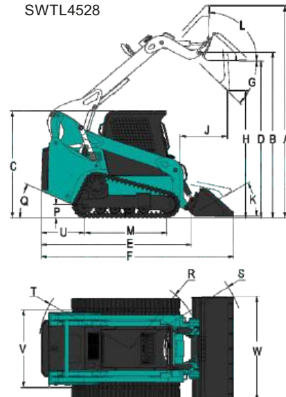
SWTL Series SWTL4528
